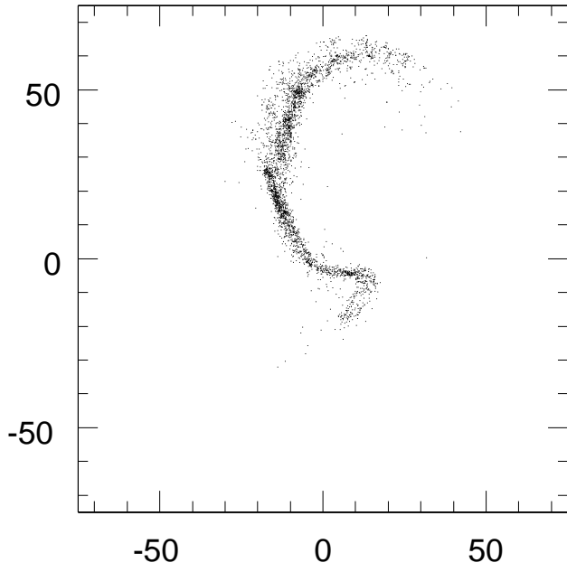
E_{\text{gained}} > -1.25 - \Phi_{\text{init}}
