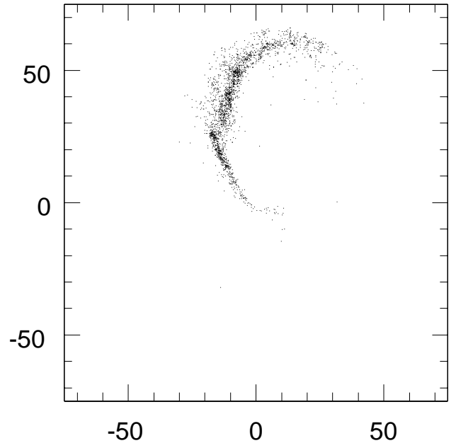
E_{\text{gained}} > -1 - \Phi_{\text{init}}
