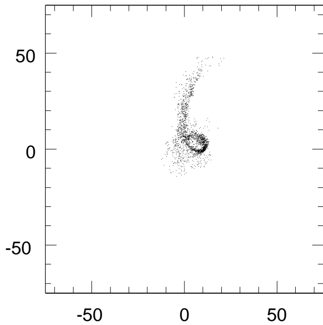
E_{\text{gained}} > -2.25 - \Phi_{\text{init}}
