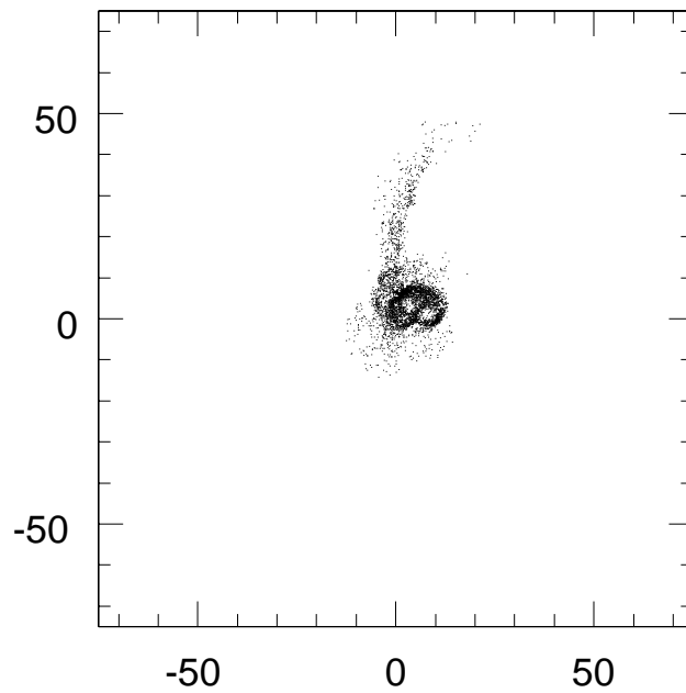
E_{\text{gained}} > -2 - \Phi_{\text{init}}
